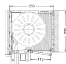
VEKAVARIANT 235 mm Revision unten
