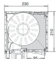
VEKAVARIANT 210 mm Revision unten
